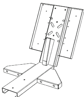
DSD-9620UK MONITOR STAND (2)
