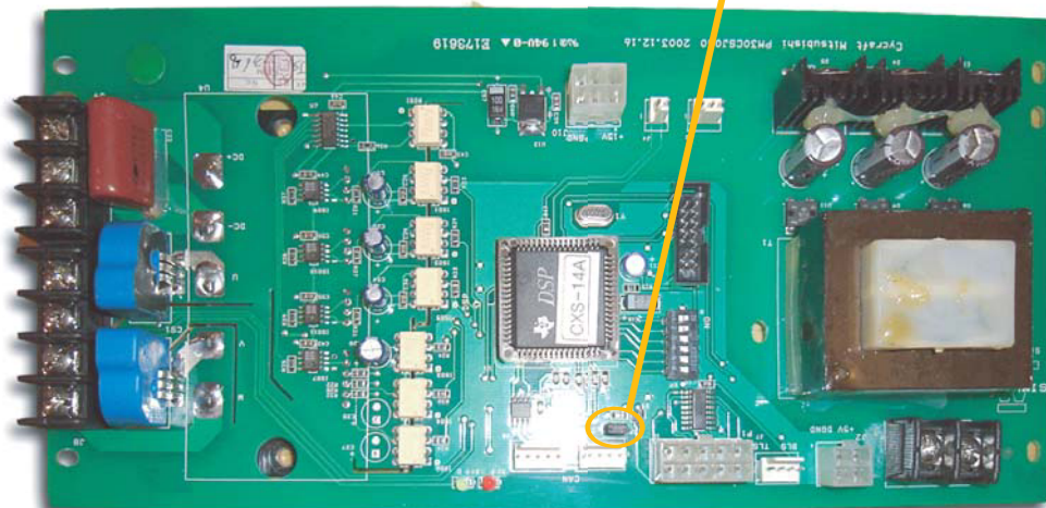
TOP VIEW OF "SERVO CONTROL BD, MITSUBISHI"
